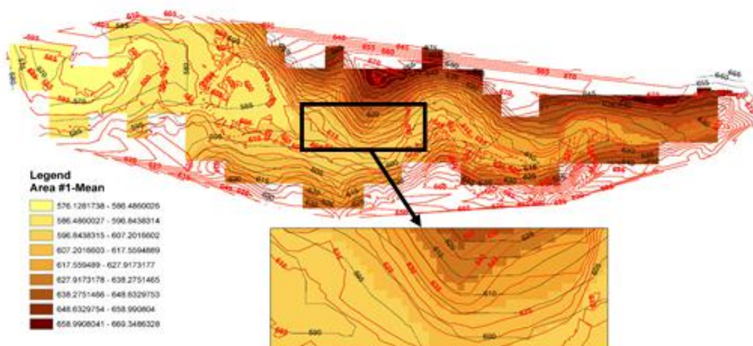
Figure-11: mean elevations in study area-1
